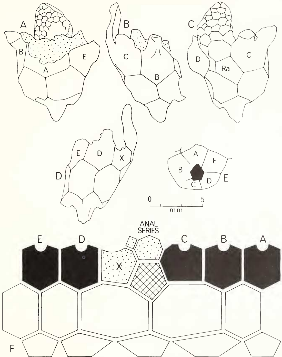
TEXT-FIG. 1. Euspirocrinus girvatensis sp. nov. A-E, HM E3499; holotype; camera lucida drawings of internal mould of the dorsal cup. A, A ray central. B, BC interray central. C, CD interray central. D, D ray central. E, basal view (axial canal of column shaded). Key: A to E, Carpenter rays; Ra, radianal; X, anal X plate. F, schematic plating diagram of the dorsal cup. Infrabasals and basals unshaded; radials black; radianal cross-hatched; anal series stippled.
